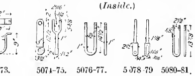
Figs. 5070-71. END AND CENTER AXLE-GUARDS.
